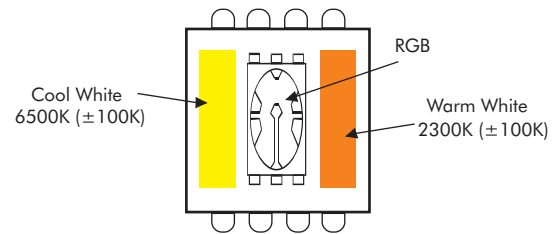
New RGBCCT - 5 Color Chips in 1 LED
